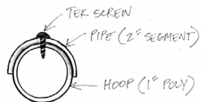
HOOP CROSS SECTION
