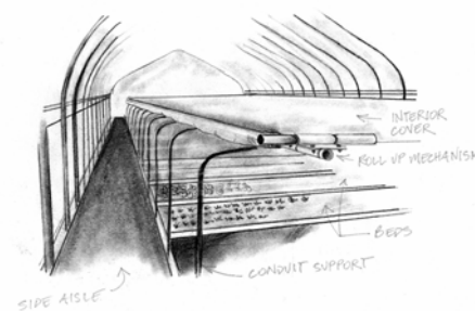
DIAGRAM 12. INTERIOR COVER SUSPENDED OVER EMT CONDUIT SUPPORTS
